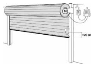
Example of installation on roller door with control panel and RADIOBANDRU .
